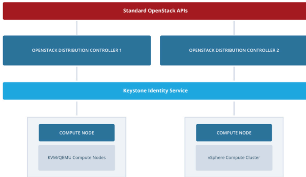
Figure 2: Example of Multi-Distribution/Multi-Hypervisor Architecture
