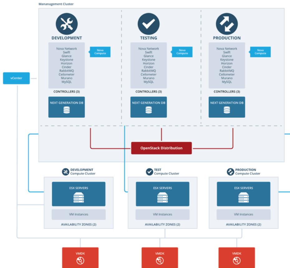
Figure 3: Example OpenStack Distribution Supporting VMware Infrastructure
